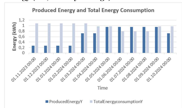
Figure 3 “Brownfield” Total Energy Consumption System 2 (130 qm²)
