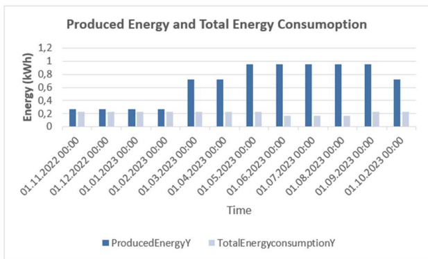
Figure 7 “Greenfield” Total Energy Consumption System 2 (130 qm 2 )
