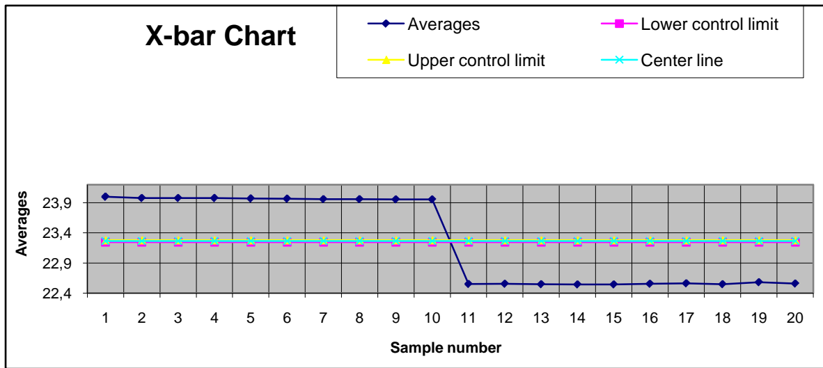
Fig.5 Chart of the XBar-R measurements.
