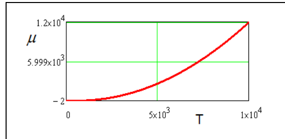
Figure 3. Argument of Bessel functions \mu = k_x p_\perp / \gamma \dot{\psi}, \varepsilon = 2, k_x = 0.1
