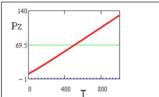
Figure 6. Time dependence of the longitudinal momentum of a particle under the following initial conditions: \varepsilon = 1; k_x = 0.1; p_x = p_y = 0.1; p_z = 10; x = y = 0; z = 1
