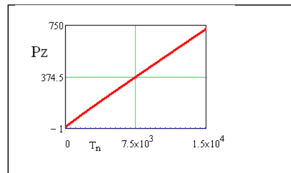
Figure 8. Time dependence of the longitudinal momentum of a particle under the following initial conditions: \varepsilon = 0.5, p_z(0) = 10, k_x = 0.1, \varepsilon k_x = 0.05; \gamma \dot{\psi} \approx \frac{1}{2 p_z} = 0.05; \varepsilon k_x = \gamma \dot{\psi}
