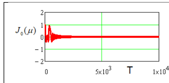
Figure 4. The Bessel functions themselves decrease rapidly \mu = k_x p_\perp / \gamma \dot{\psi}, \varepsilon = 2, k_x = 0.1
