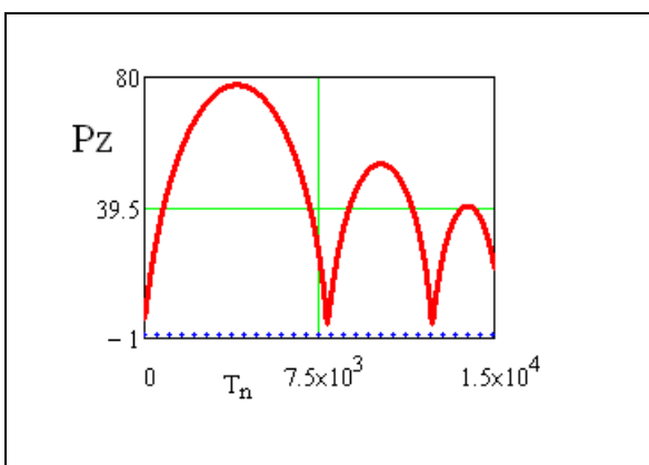
Figure 7. Time dependence of the longitudinal momentum of a particle under the following
