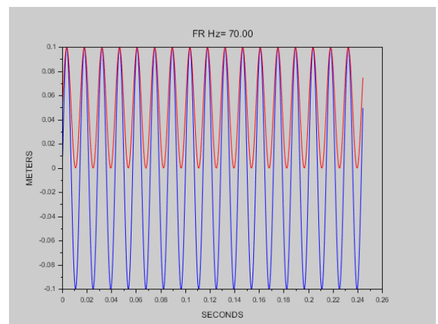
Fig. 3. Displacements
