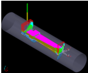
Figure 6. Raster finishing
