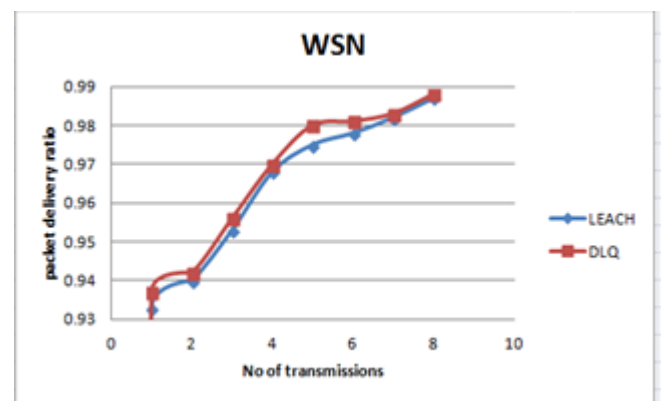
Fig. 8. Packet Delivery ratio vs. No. of transmissions
