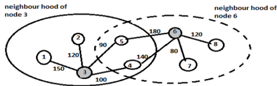
Fig. 4. Example of a WSN with LQI values
