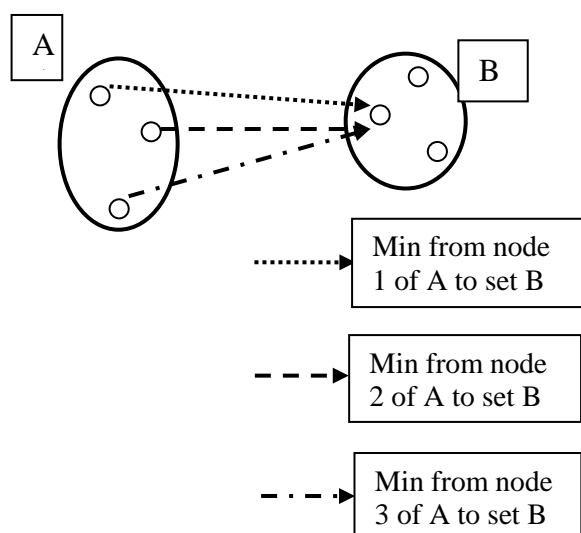
Fig. 3. Example of calculating Hausdorff distance
