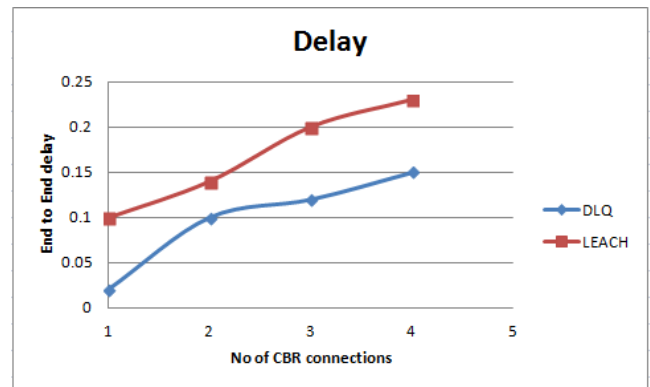
Fig. 11. End to end delay Vs No of CBR connections
