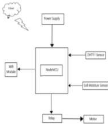
Block Diagram of Smart irrigation system
