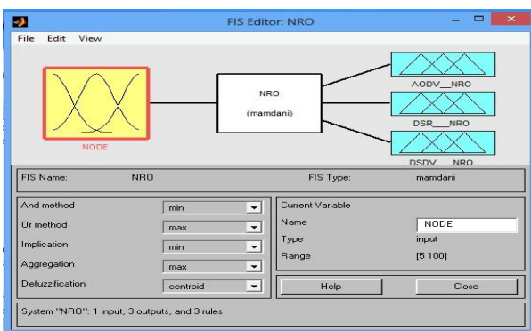
Fig. 2: General model of fuzzy expert System for evaluation of three routing Protocol.
