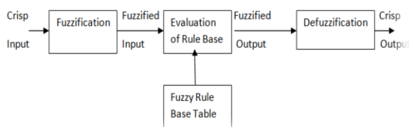
Figure 1: Fuzzy Logic Inference system
