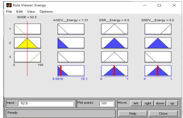
Fig. 12: Result of simulation with 50 nodes output of Energy
