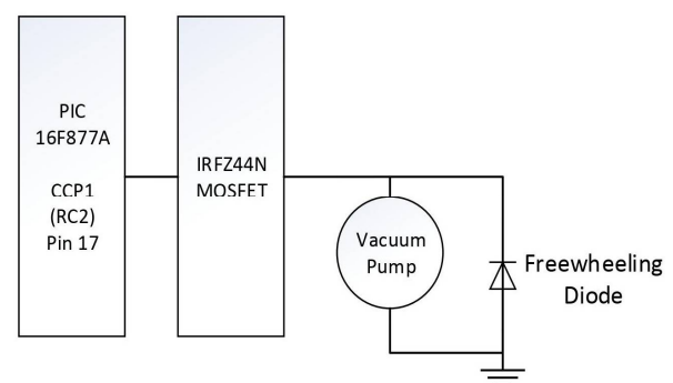
Fig. 2 Block Circuit connection of Biomedical Suctioner
